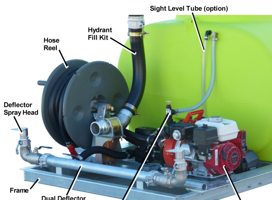
Figure 2 – Component Identification
