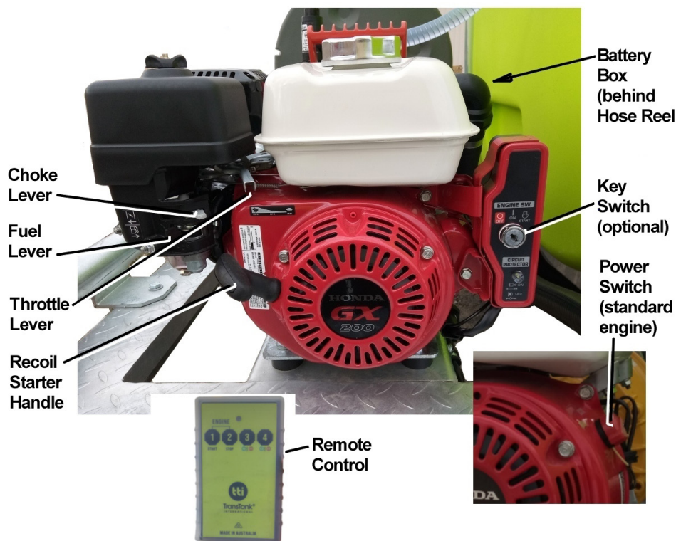
Figure 3 – Engine Start-up (Petrol Engine shown)
