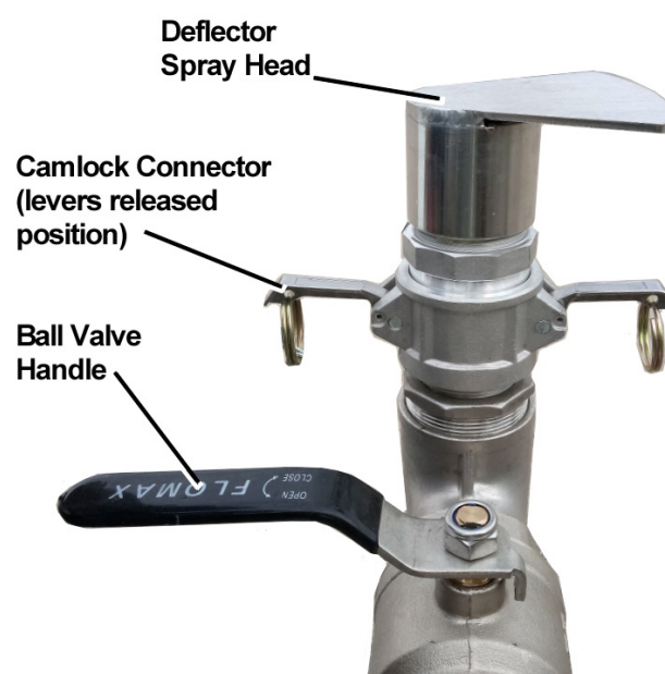
Figure 8 – Water Deflector Spray Head
