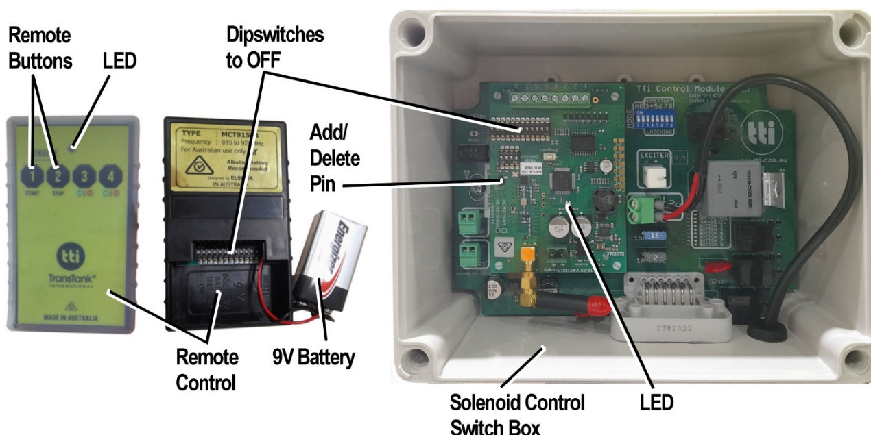
Figure 13 – Solenoid Control Switch and Remote Control
