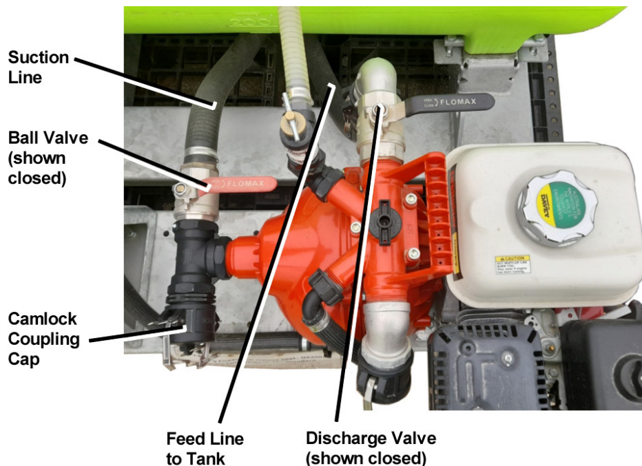
Figure 4 – Tank Filling Operation
