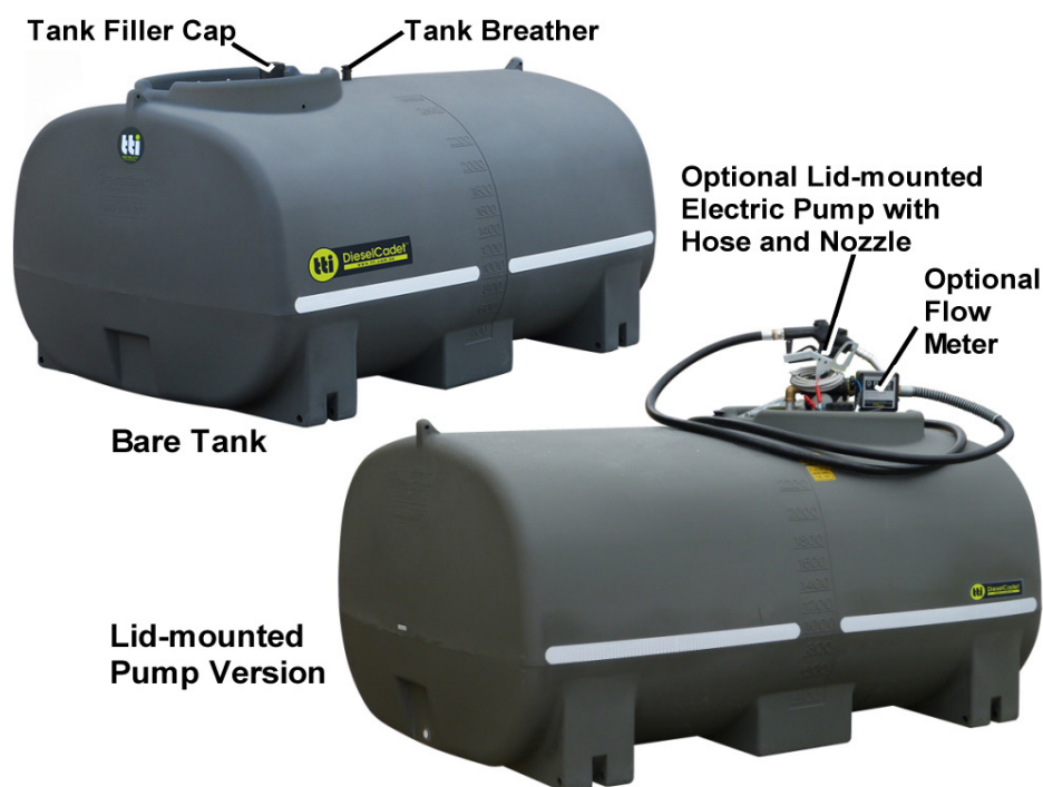
Figure 1 – Component Identification – DieselCadet (no frame versions)
