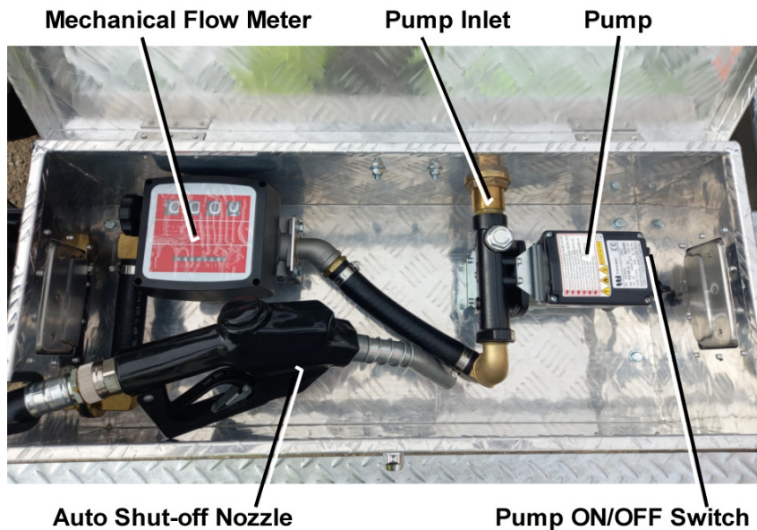
Figure 5 – Transfer Operation – Electric Pump
